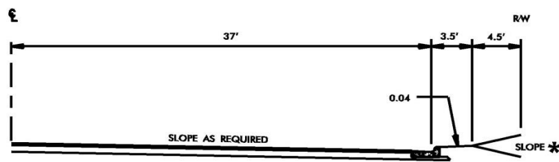
2'-6" CURB & GUTTER
