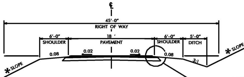
RESIDENTIAL LOCAL ROAD
