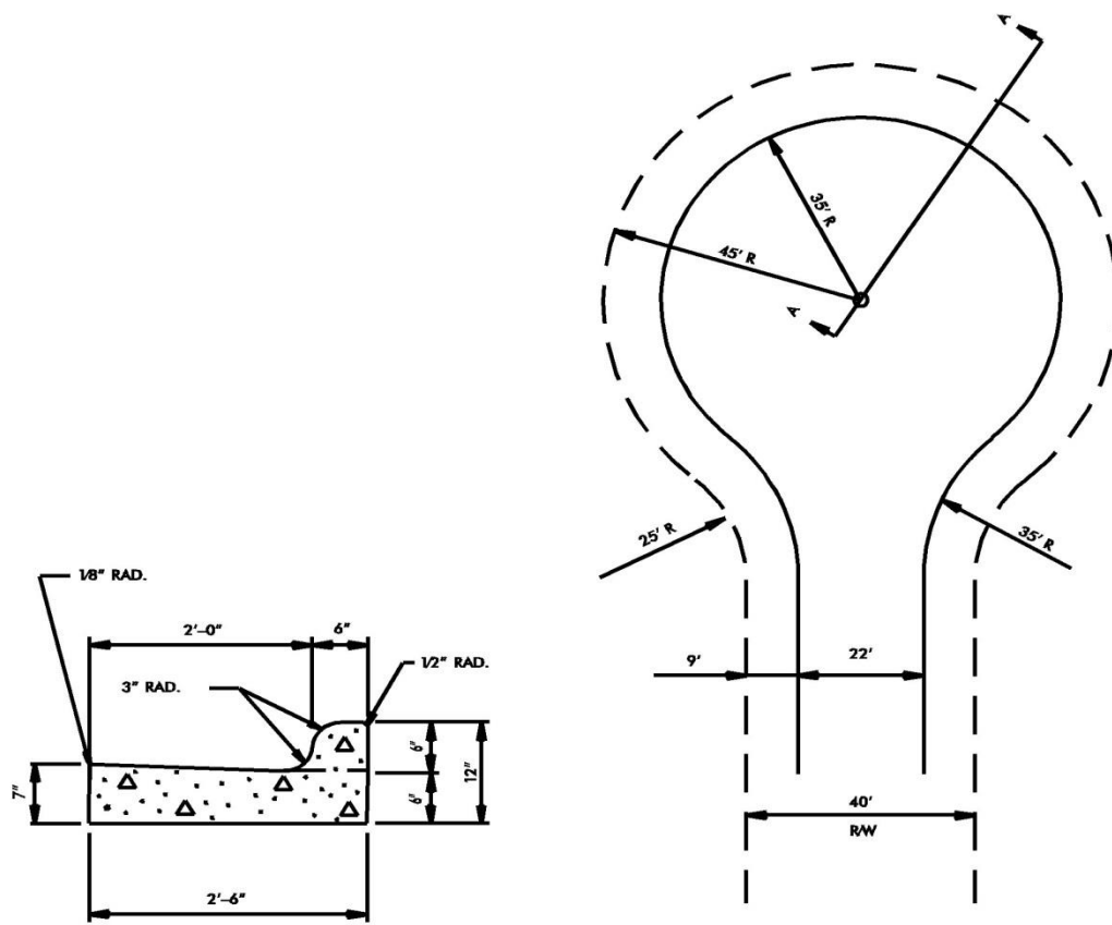
2'-6" CURB & GUTTER
